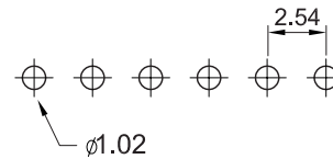
Recommended P.C. Board Hole Layout
